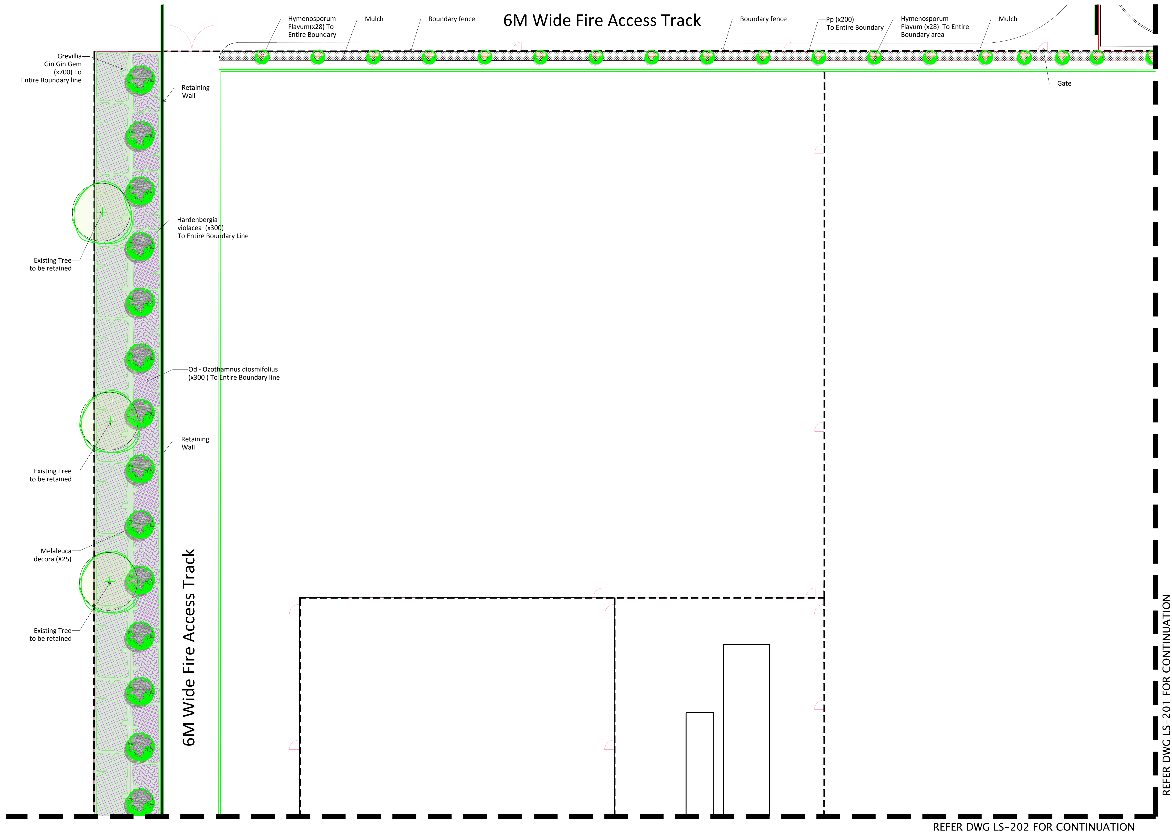
LANDSCAPE PLAN SCALE 1:200 @ A1
